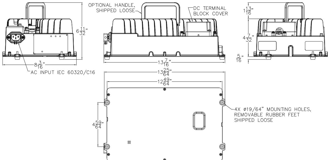
Figure 2-2: Charger Dimensions and Mounting Hole Locations
